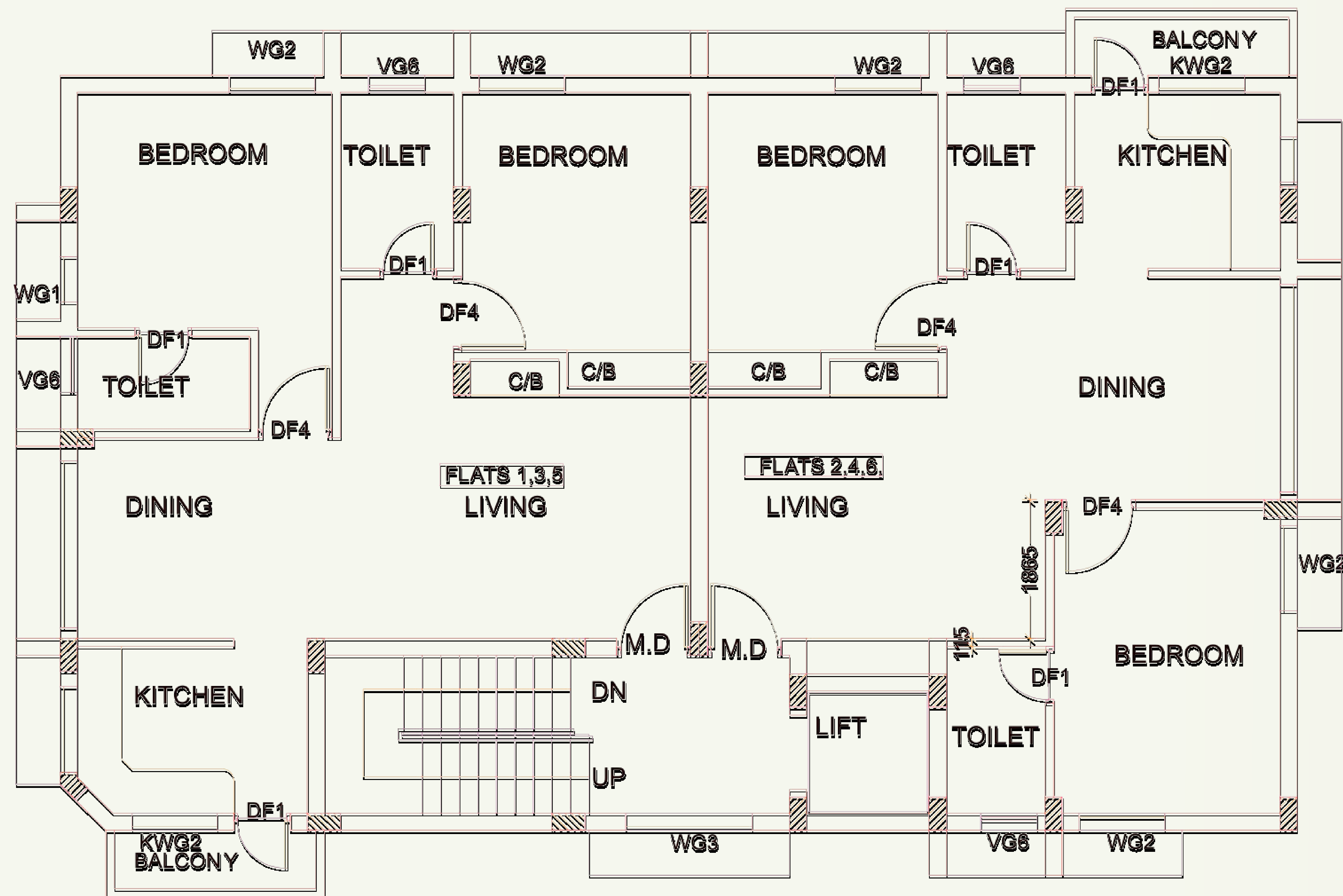
TYPICAL FLOOR PLAN(1,2,3)
